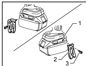
1. Groove 2. Hook 3. Screw
