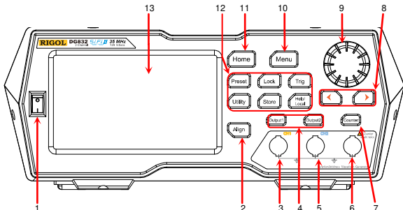
Figure 1 Front Panel
