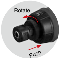
▲ Spindle Lock Design - Push and Rotate to Lock
