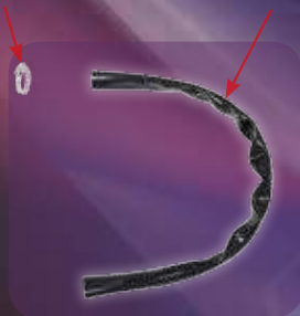
50-500232-12S Overhose Assembly (Optional)
