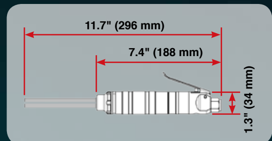
SM-106NS-3 3 mm Needle Scaler
