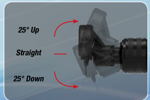
▲ 3 Position Flex Head
